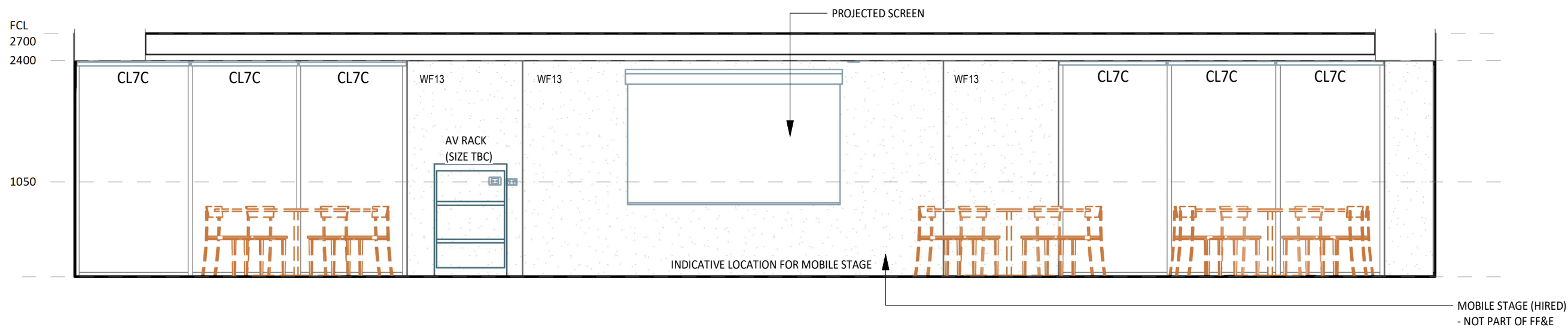
1 ELEVATION DETAIL 1 : 50
